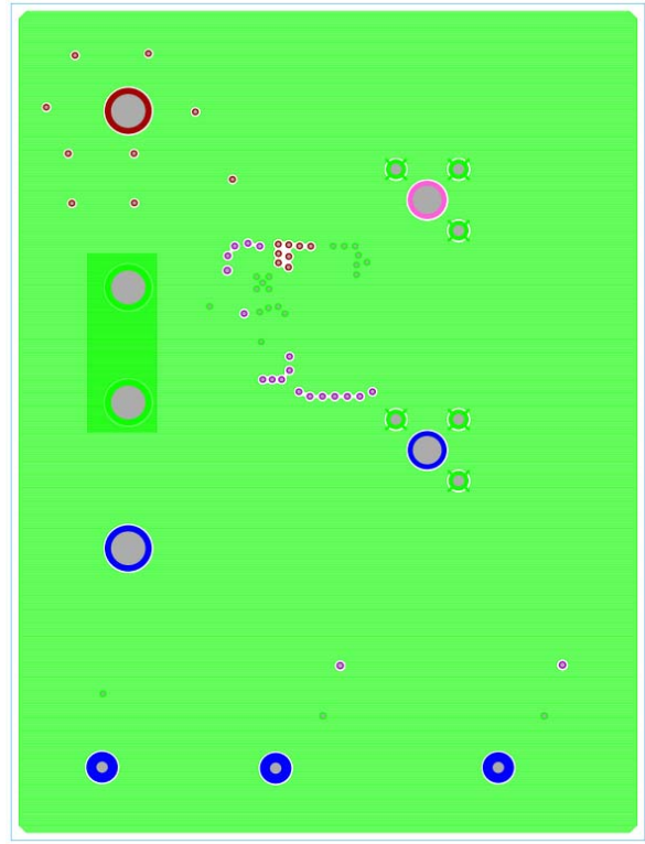
FIGURE 5. LAYER 2 PCB
