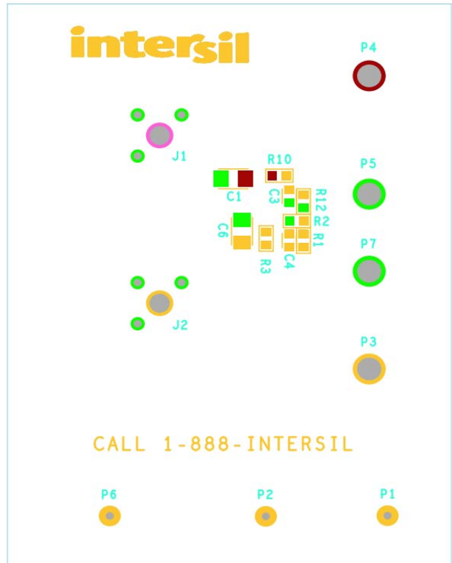
FIGURE 3. BOTTOM LAYER SILKSCREEN
