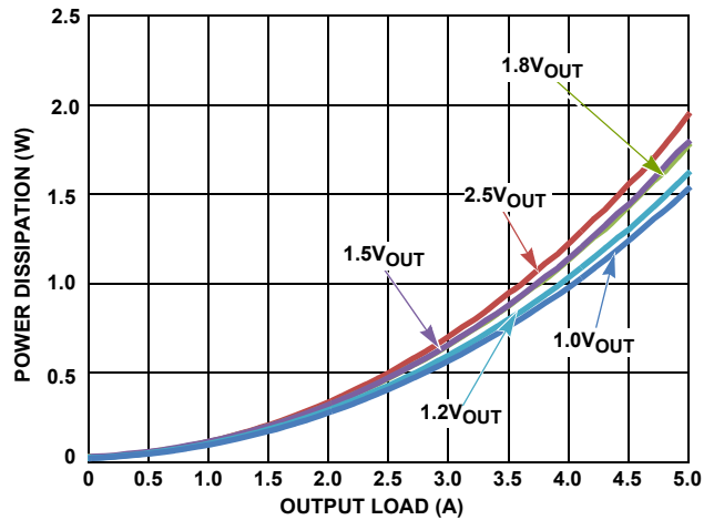
FIGURE 11. POWER DISSIPATION vs LOAD (3V IN ; SYNC = VDD)
