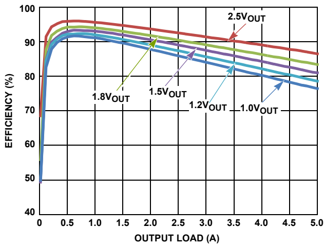
FIGURE 10. EFFICIENCY vs LOAD (3V IN ; SYNC = VDD)
