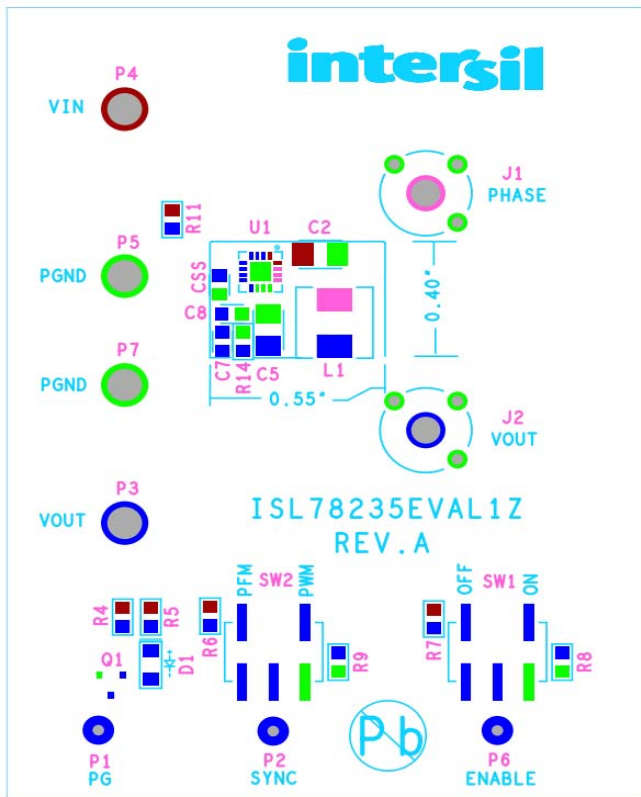
FIGURE 2. TOP LAYER SILKSCREEN
