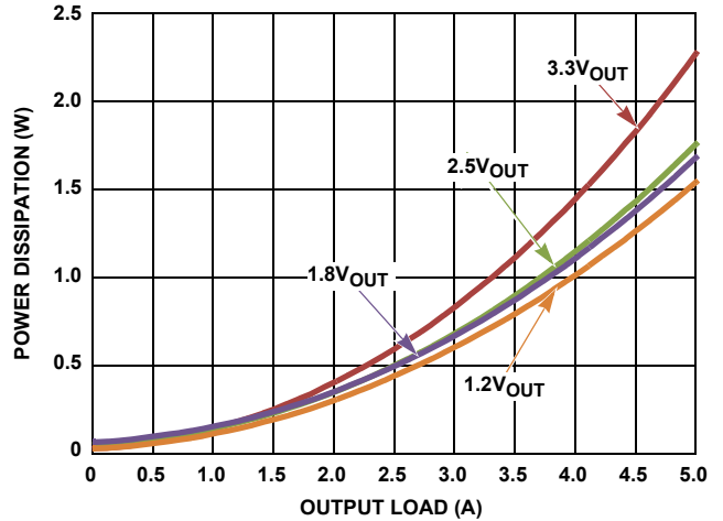
FIGURE 9. POWER DISSIPATION vs LOAD (5V IN ; SYNC = VDD)
