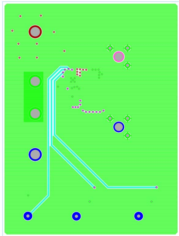
FIGURE 6. LAYER 3 PCB
