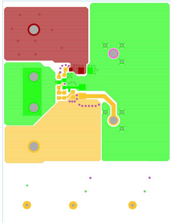
FIGURE 7. LAYER 4 PCB
