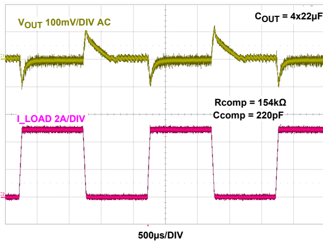
FIGURE 12. LOAD TRANSIENT 0A TO 5A; 0.5A/μs (SYNC = GND)
