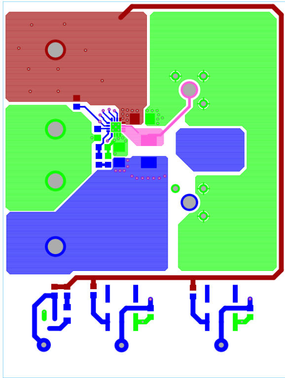
FIGURE 4. LAYER 1 PCB
